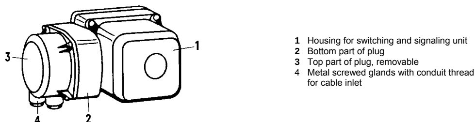
Fig. 3 : Housing for switching and signaling unit and plug housing ( design for S - SIWI series )
