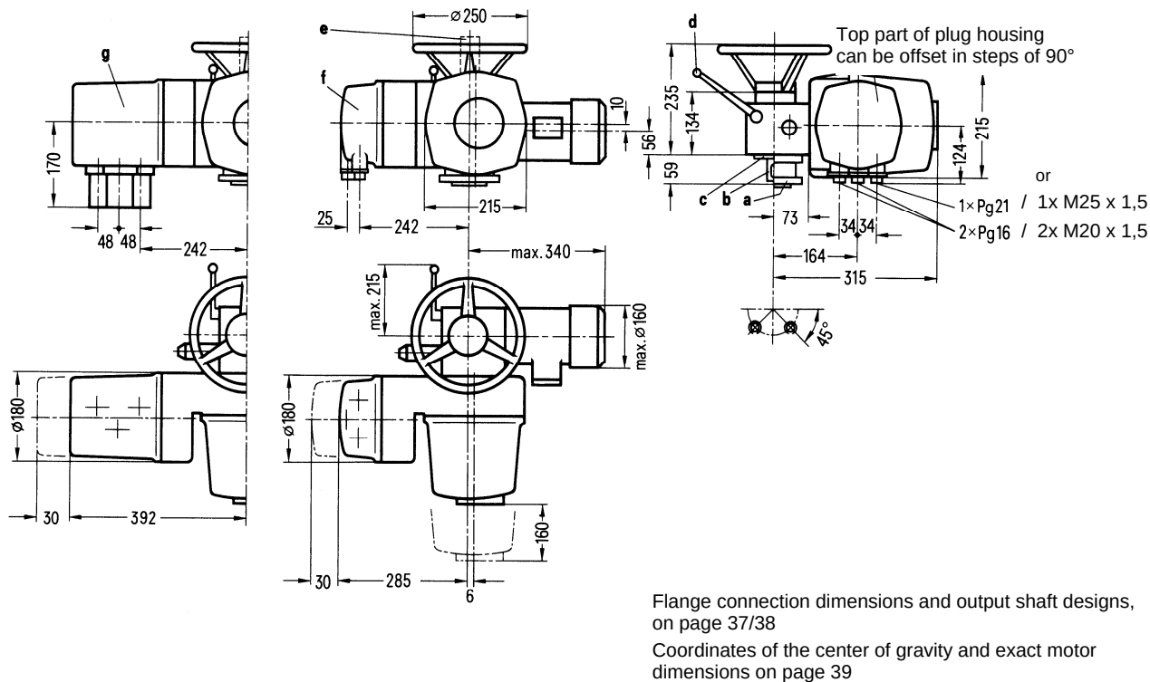
Fig. 6 Electric rotary actuators M76361 – C and M76371 – C, size 0 to DIN 3210 / F10 to EN ISO 5210
